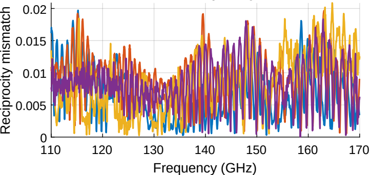
Hold-out DIAG reciprocity residuals
